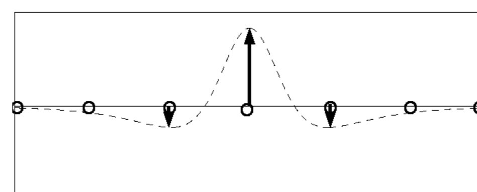
Figure 2. Even-parity bright-type breather solution, given by Eq. (??).
