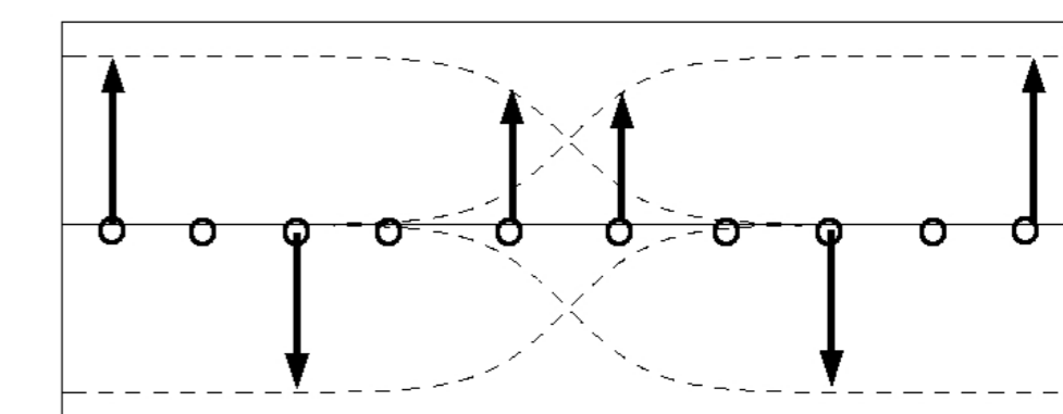
Figure 4. Grey type dust lattice excitation: successive dust grain displacements.
