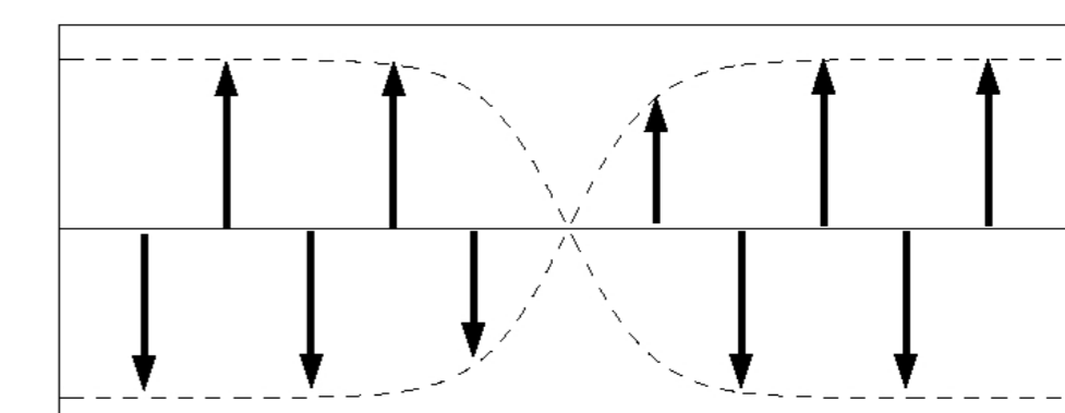
Figure 3. Dark type dust lattice excitation: successive dust grain displacements. Focusing in the middle of the Brillouin zone, i.e. at k = \pi/2r_0 (where odd sites remain at rest, while even ones oscillate out of phase; cf. the analysis in [?, ?]), one obtains [?, ?] the pattern
