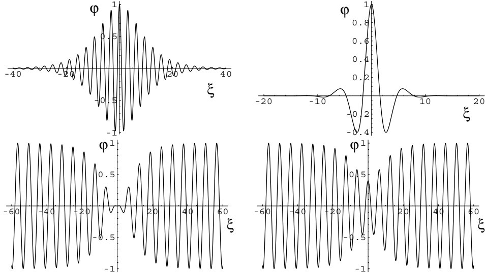
FIG. 1: A representation of wave packets modulated by solutions of the NLS equation. These envelope excitations are of the: (a, b) bright type ( PQ > 0 , pulses); (c) dark type, (d) gray type ( PQ < 0 , voids). Notice that the amplitude never reaches zero in (d).
