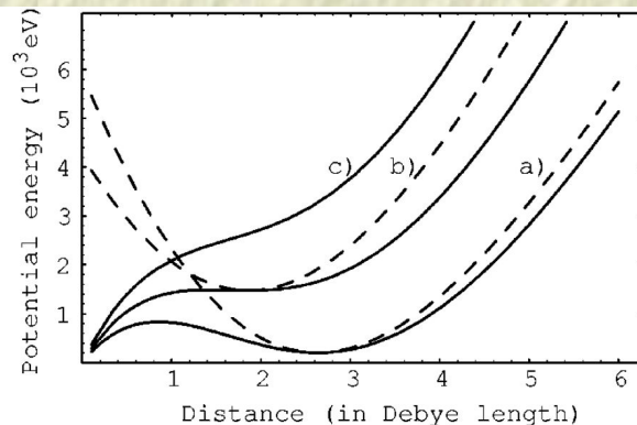
FIG. 8. The total interaction energy U_{\text{tot}} as a function of the distance h = z/\lambda_D from the electrode for the different sizes of a dust particle: (a) a = 0.35 \times 10^{-3} cm; (b) a = a_{\text{cr}} = 0.372 \times 10^{-3} cm; and (c) a = 0.4 \times 10^{-3} cm. The dashed lines correspond to the case of a charge constant at the equilibrium (or marginal equilibrium) position: (a) Q = -5.42e \times 10^3 and (b) Q = -4.93e \times 10^3 .
