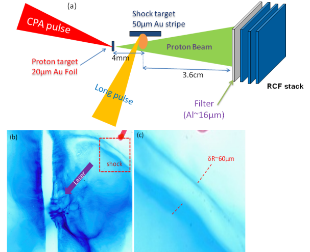
Fig. 1: (a) The schematic of experimental setup, with time of flight arrangement of proton probing (b) Proton Image of the interaction of nanosecond pulse with 50\mu\text{m} Au stripe, showing shock waves in laser ablating plasma, the arrow shows the direction of the laser (c) zoom of observed structure.
