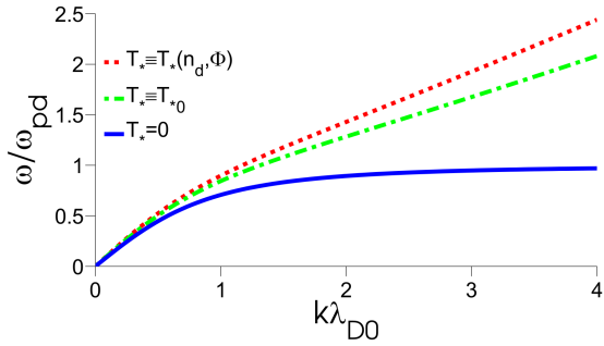
FIG. 5: (Colour online) The normalised dispersion relation for three different models of dust-acoustic waves. Here we have n_{i0} = 7 \times 10^{13} \text{ m}^{-3} , n_{e0} = 4 \times 10^{13} \text{ m}^{-3} , k_B T_i = 0.3 \text{ eV} , k_B T_e = 8 \text{ eV} , m_d = 1 \times 10^{-13} \text{ kg} , r_d = 0.2 \text{ } \mu\text{m} , and \sigma = 1.3732 \times 10^{-5} .
