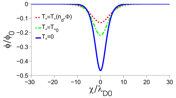
FIG. 6: (Colour online) Normalised solitary wave structures for three different models. Here we have n_{i0} = 7 \times 10^{13} \text{ m}^{-3} , n_{e0} = 4 \times 10^{13} \text{ m}^{-3} , k_B T_i = 0.3 \text{ eV} , k_B T_e = 8 \text{ eV} , m_d = 1 \times 10^{-13} \text{ kg} , r_d = 0.2 \text{ } \mu\text{m} , \sigma = 1.3732 \times 10^{-5} and \tilde{V} = 1.2 .
