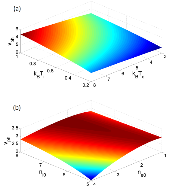
FIG. 2: (Colour online) The phase velocity, v_{ph} (cm/s) of the dust-acoustic waves studied in this investigation, as functions of (a) the temperatures (eV), and (b) the densities ( \times 10^{13} \text{ m}^{-3} ) of the Maxwellian species. In both plots we have m_d = 1 \times 10^{-13} \text{ kg} , r_d = 0.2 \text{ }\mu\text{m} and \sigma = 1.3732 \times 10^{-5} . In (a) we have n_{i0} = 7 \times 10^{13} \text{ m}^{-3} , n_{e0} = 4 \times 10^{13} \text{ m}^{-3} and in (b) we have k_B T_i = 0.3 \text{ eV} , k_B T_e = 8 \text{ eV} .
