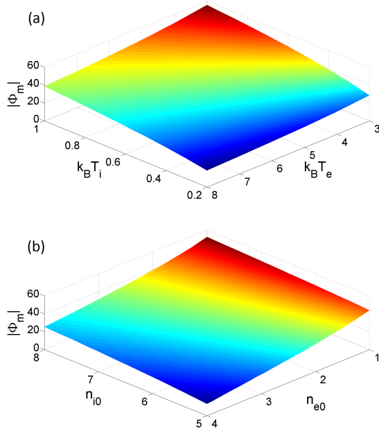
FIG. 3: (Colour online) The amplitude, |\Phi_m| (mV) of the potential perturbations associated with the solitary waves studied in this investigation, as functions of (a) the temperatures (eV), and (b) the densities ( \times 10^{13} \text{ m}^{-3} ) of the Maxwellian species. In both plots we have m_d = 1 \times 10^{-13} \text{ kg} , r_d = 0.2 \text{ }\mu\text{m} , \sigma = 1.3732 \times 10^{-5} and \delta V = 2 \text{ mm/s} . In (a) we have n_{i0} = 7 \times 10^{13} \text{ m}^{-3} , n_{e0} = 4 \times 10^{13} \text{ m}^{-3} and in (b) we have k_B T_i = 0.3 \text{ eV} , k_B T_e = 8 \text{ eV} .
