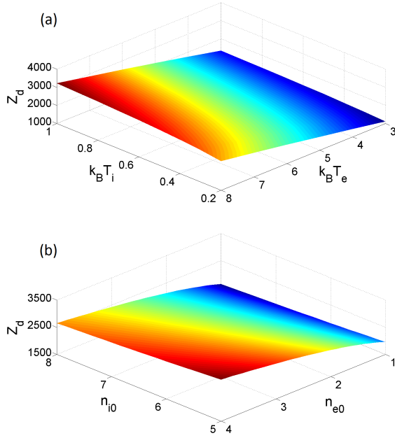
FIG. 1: (Colour online) The charge number of the dust particles studied in this investigation, as functions of (a) the temperatures (eV), and (b) the densities ( \times 10^{13} \text{ m}^{-3} ) of the Maxwellian species. In both plots we have m_d = 1 \times 10^{-13} \text{ kg} , r_d = 0.2 \text{ }\mu\text{m} , k_B T_d = 0.3 \text{ eV} \sigma = 1.3732 \times 10^{-5} . In (a) we have n_{i0} = 7 \times 10^{13} \text{ m}^{-3} , n_{e0} = 4 \times 10^{13} \text{ m}^{-3} and in (b) we have k_B T_i = 0.3 \text{ eV} , k_B T_e = 8 \text{ eV} .
