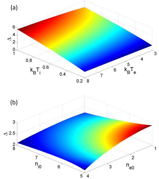
FIG. 4: (Colour online) The width, \Delta (mm) of the potential perturbations associated with the solitary waves studied in this investigation, as functions of (a) the temperatures (eV), and (b) the densities ( \times 10^{13} \text{ m}^{-3} ) of the Maxwellian species. In both plots we have m_d = 1 \times 10^{-13} \text{ kg} , r_d = 0.2 \text{ }\mu\text{m} , \sigma = 1.3732 \times 10^{-5} and \delta V = 2 \text{ mm/s} . In (a) we have n_{i0} = 7 \times 10^{13} \text{ m}^{-3} , n_{e0} = 4 \times 10^{13} \text{ m}^{-3} and in (b) we have k_B T_i = 0.3 \text{ eV} , k_B T_e = 8 \text{ eV} .
