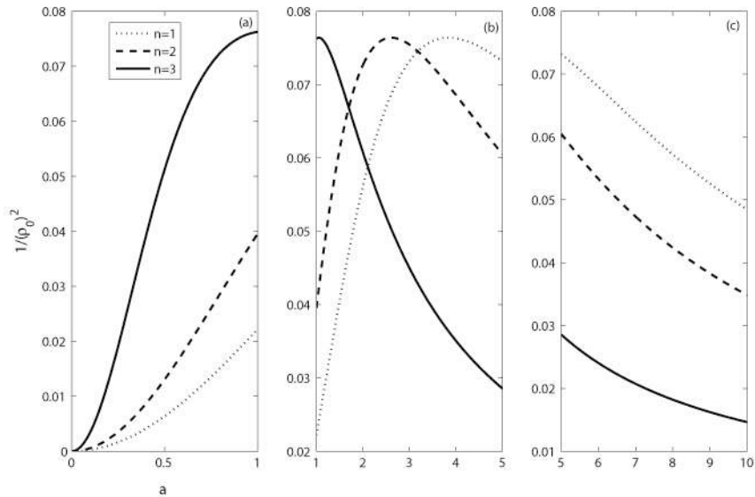
FIG. 4: Critical Curves of DHG laser pulses.
