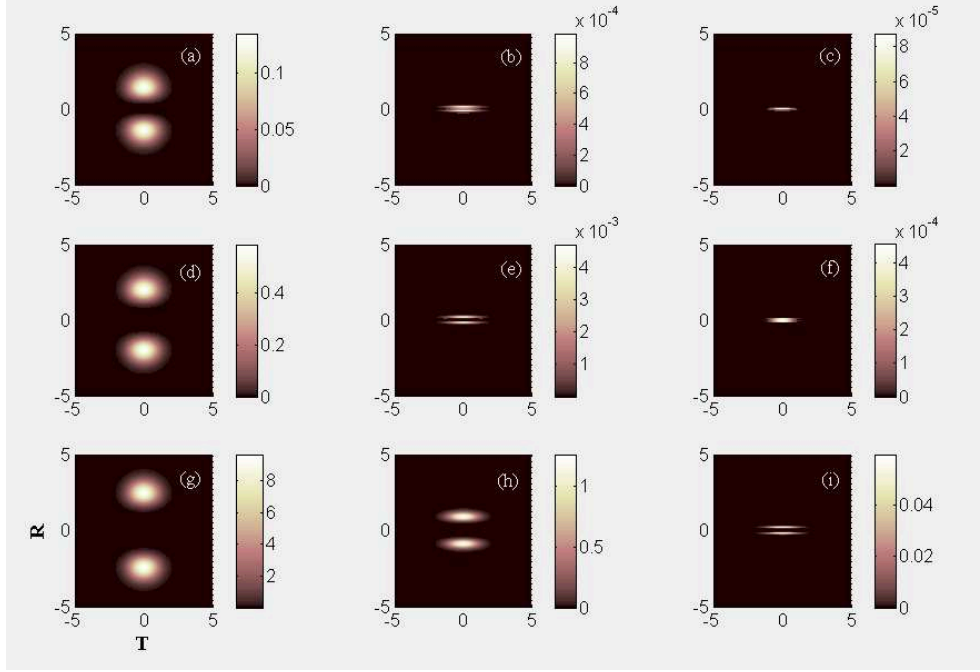
FIG. 3: (Color online) DHG pulse evolution: the variation of the normalized intensity with radial distance r and time t is shown at different propagation distance (equivalent to fixed time). The results are shown for different n values: n = 1 (top row); 2 (second row); 3 (third row). The x and y axes, respectively, present the T = \tau/\tau_L in time coordinate and R = r/r_0 in space coordinate. The color bar shows the variation in the normalized intensity.
